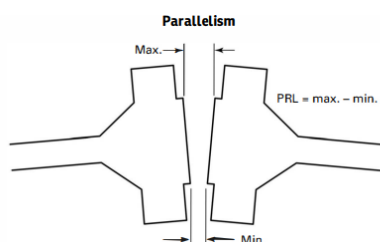
Figure 6 – Parallelism
