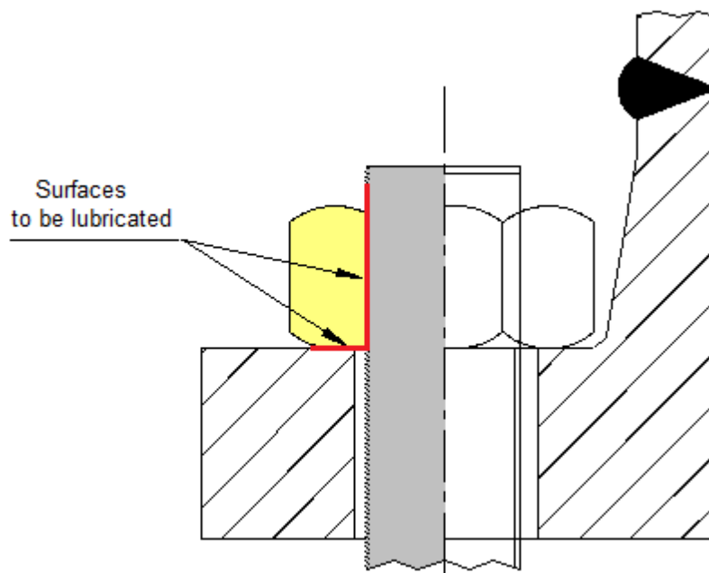
Figure 8 - Surfaces to be lubricated
