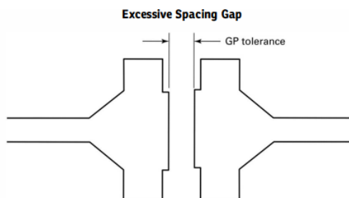
Figure 5 – Excessive Spacing Gap
