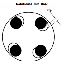
Figure 7 – Rotational Two-Hole
