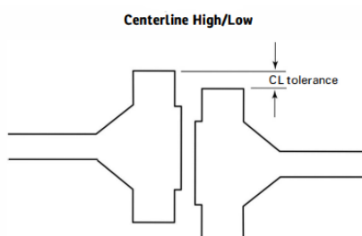
Figure 4 – Centerline High/Low
